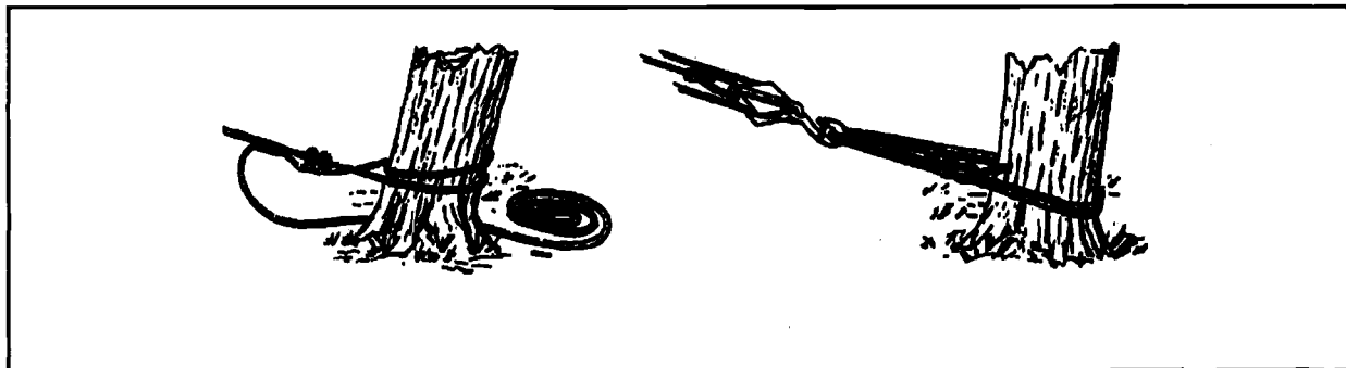
Figure 4-1. Natural anchorage (tree)
