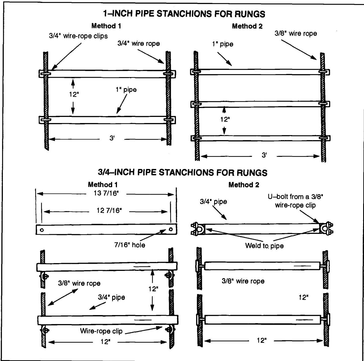
Figure 2-57. Pipe rungs
