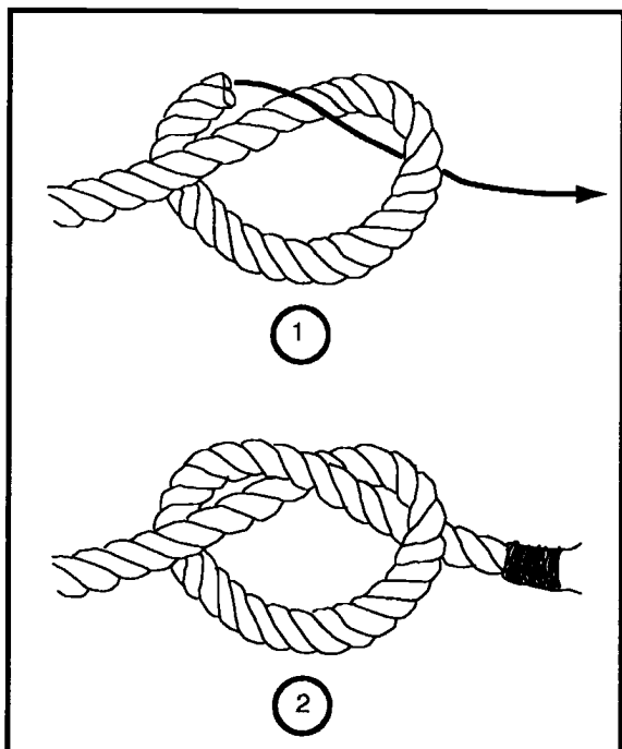
Figure 2-3. Overhand knot
