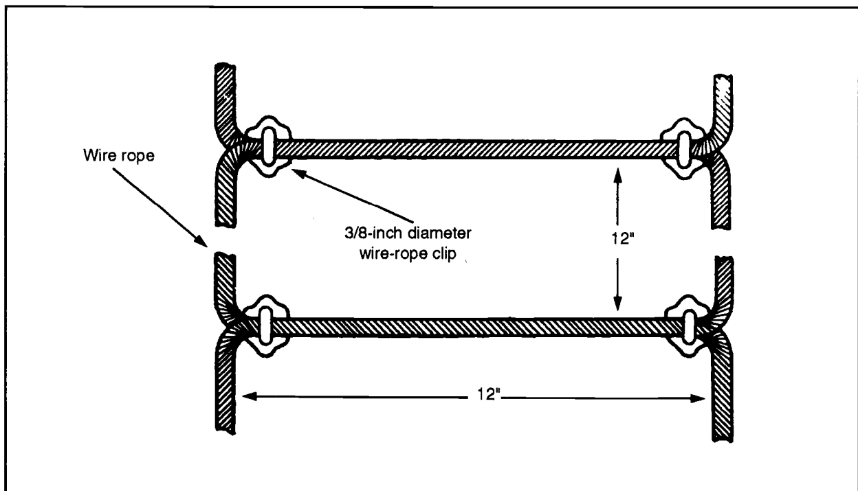
Figure 2-58. Wire-rope rungs
