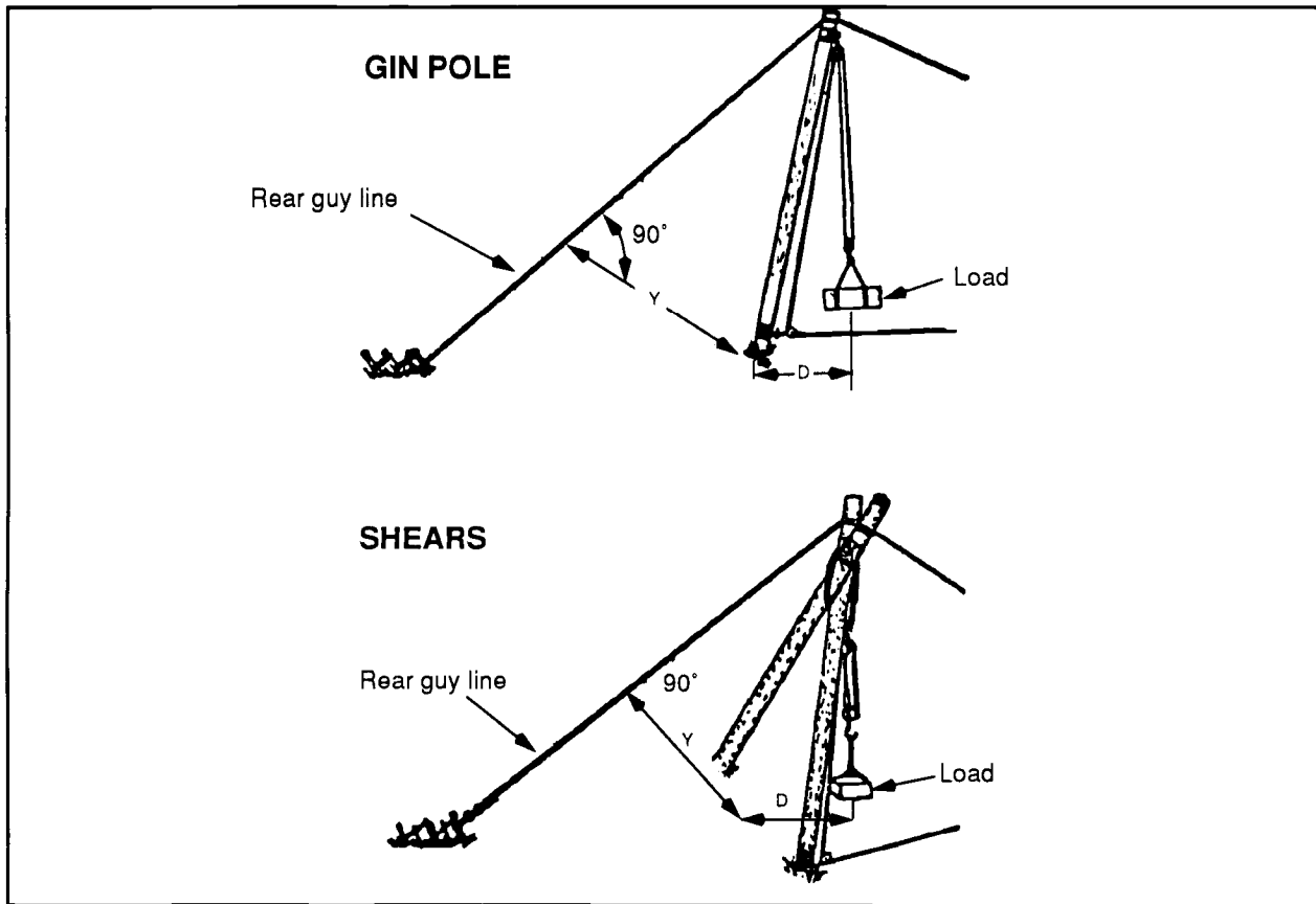
Figure 4-19. Gin pole and shears
