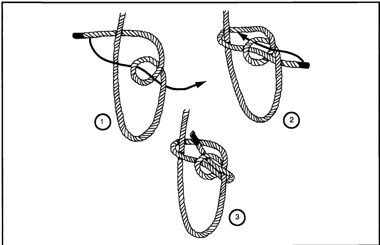
Figure 2-13. Running bowline
