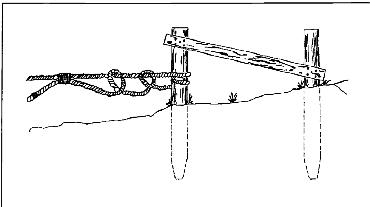
Figure 4-7. Boarded picket holdfast
