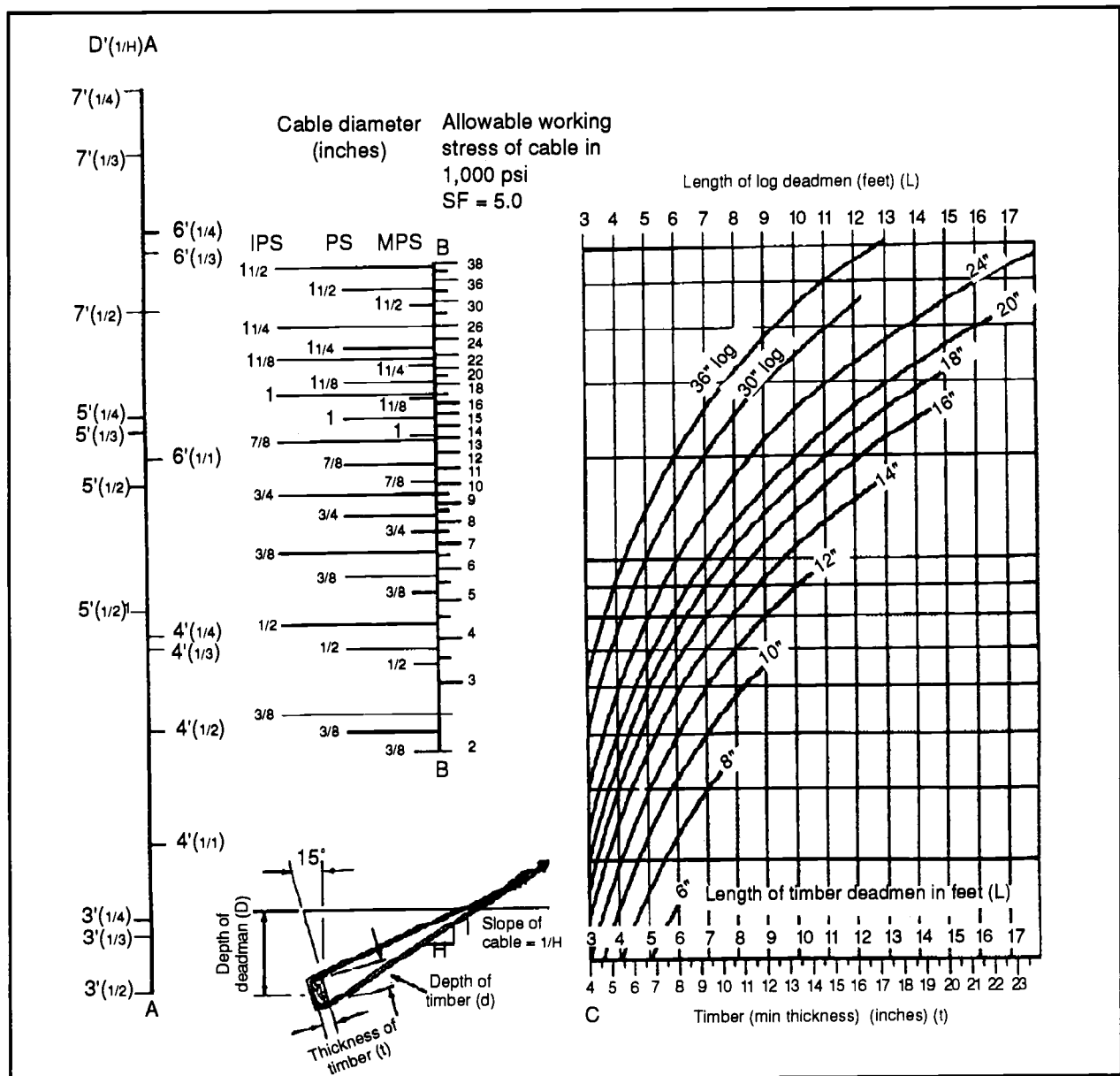
Figure 4-14. Designing a deadman
