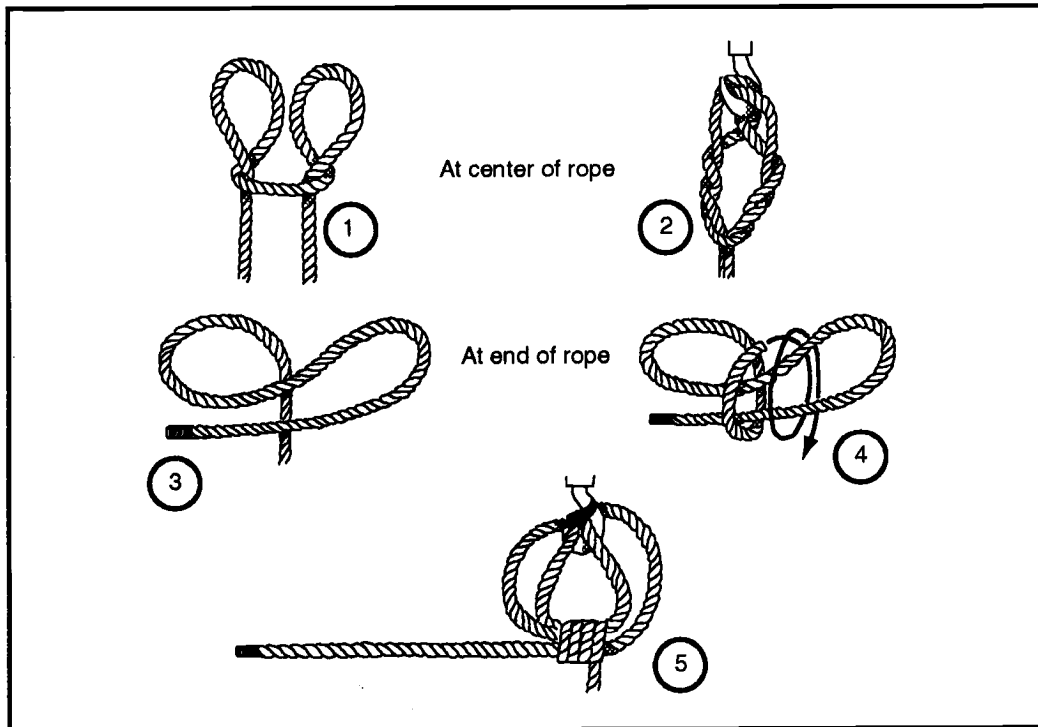
Figure 2-18. Cats-paw
