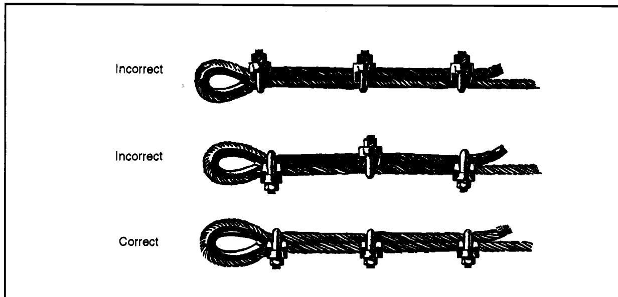
Figure 2-50. Wire-rope clips
