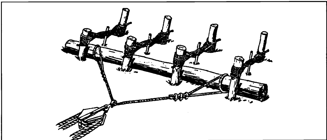
Figure 4-11. Combination log and picket holdfast
