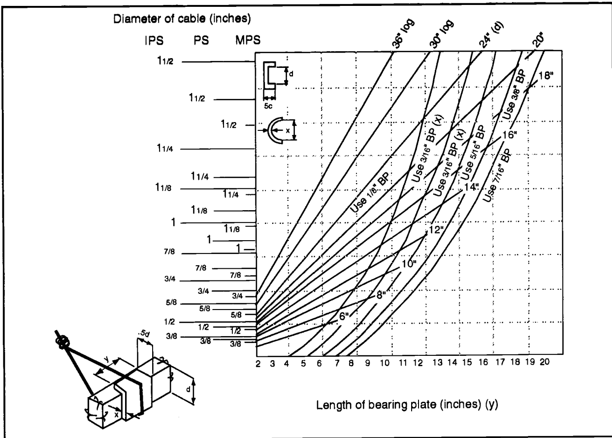
Figure 4-17. Designing a formed bearing plate
