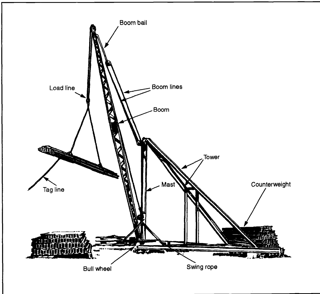
Figure 5-10. Four-ton stiff-leg derrick
