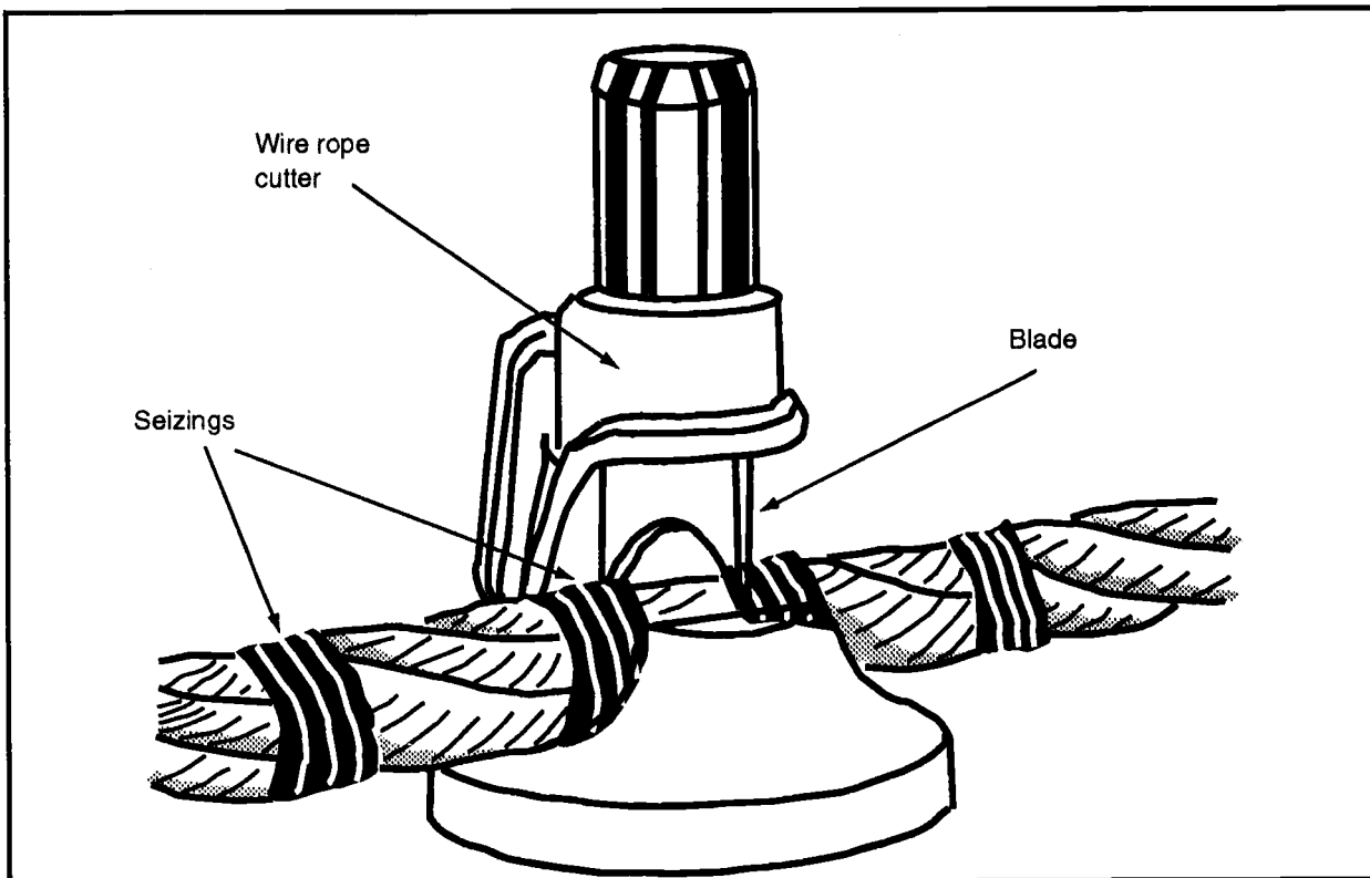
Figure 1-11. Wire-rope cutter
