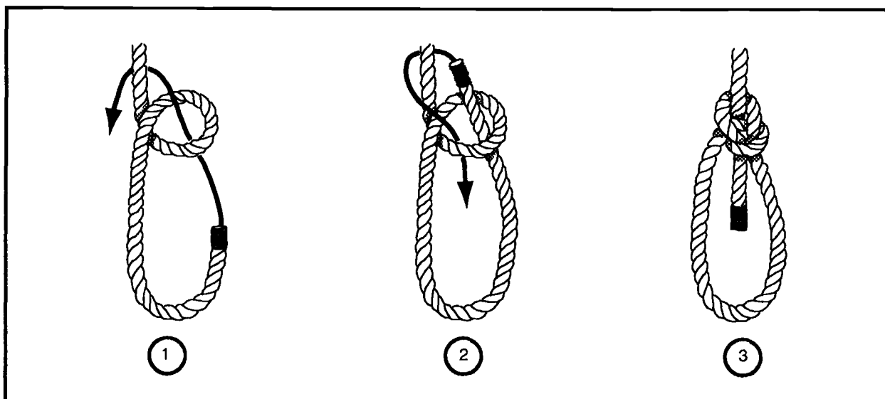
Figure 2-11. Bowline
