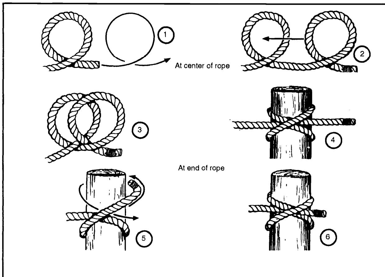
Figure 2-26. Clove hitch
