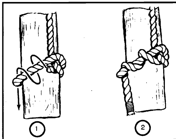
Figure 2-24. Timber hitch
