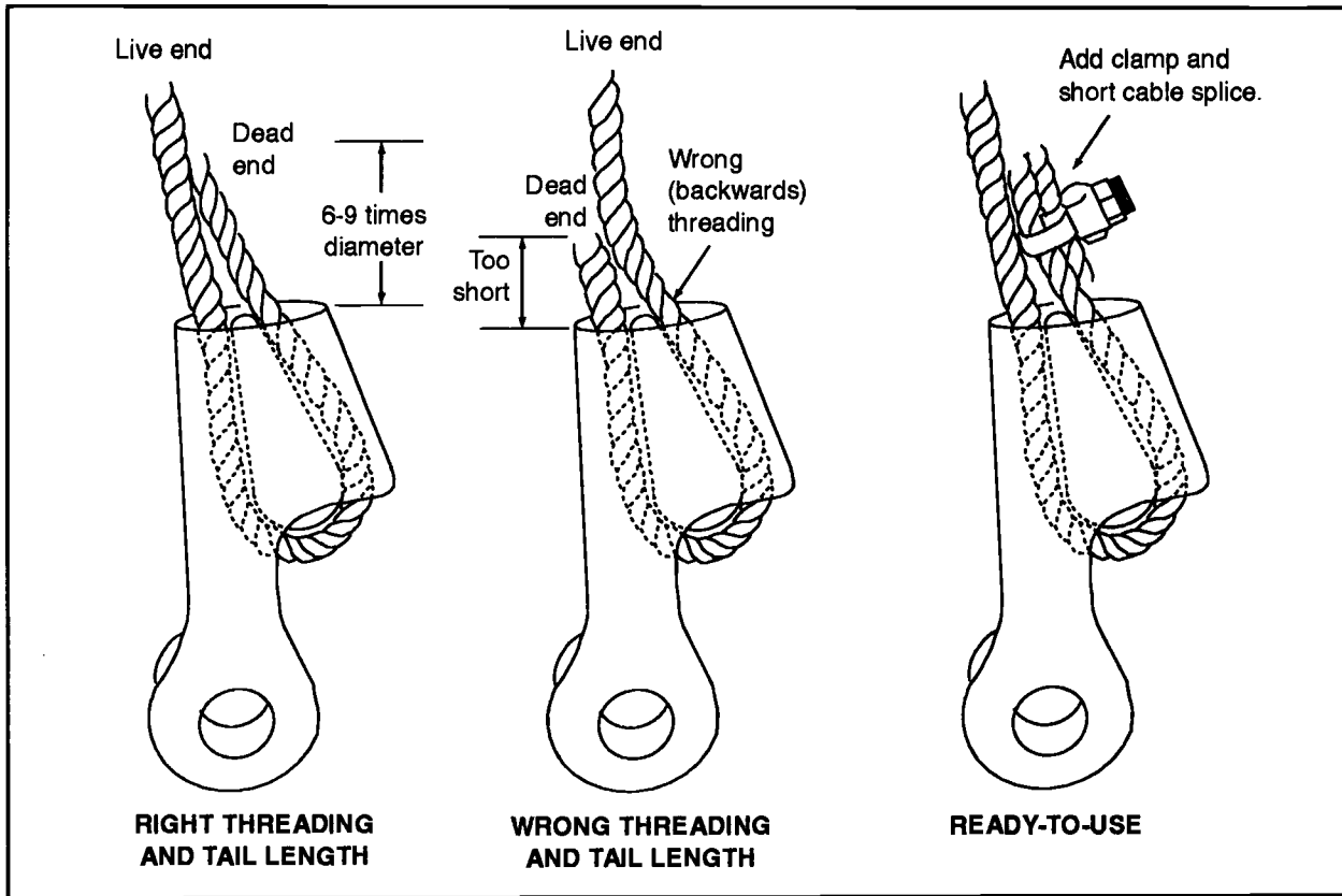
Figure 2-52. Wedge socket
