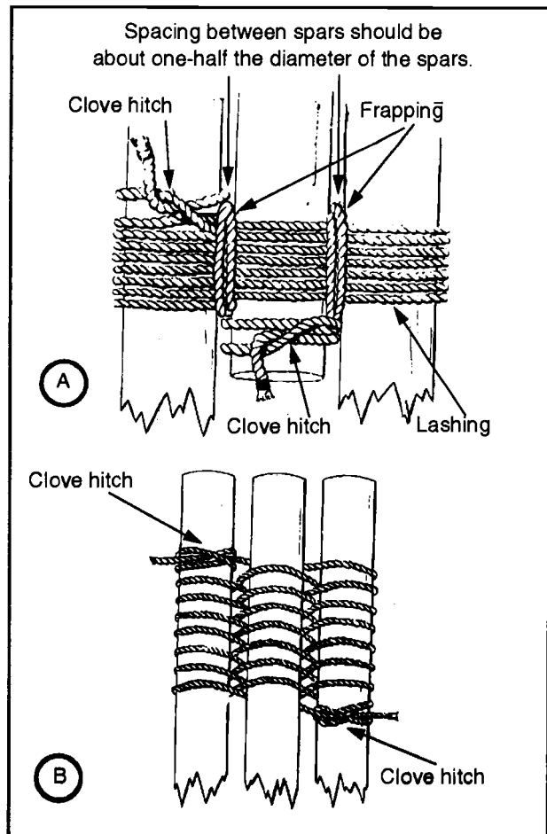
Figure 5-4. Lashing for a tripod
