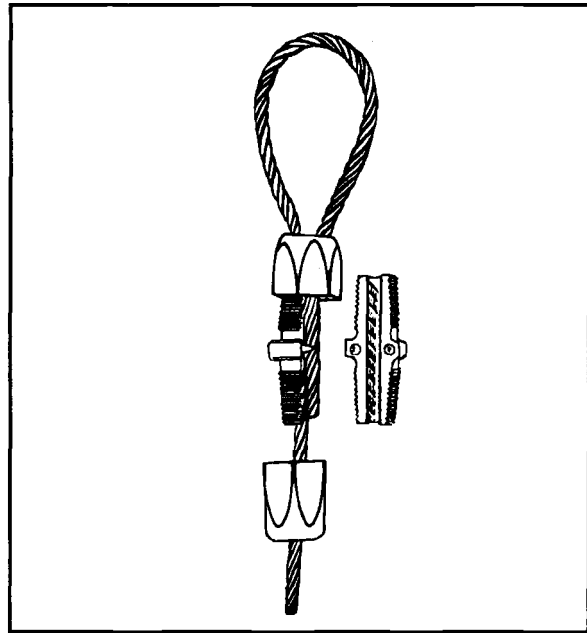
Figure 2-51. Wire-rope clamps
