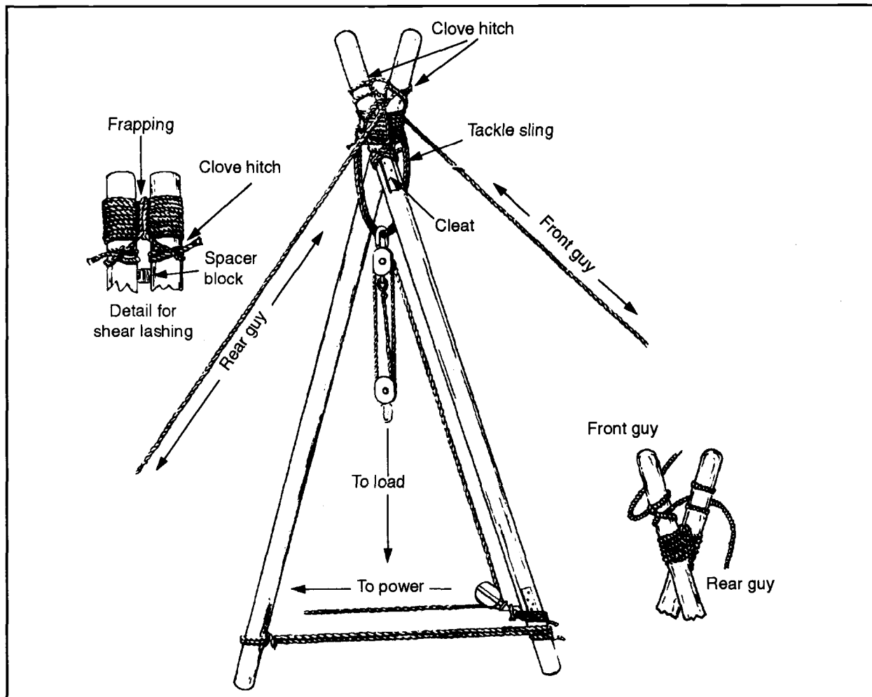
Figure 5-6. Lashing for shears
