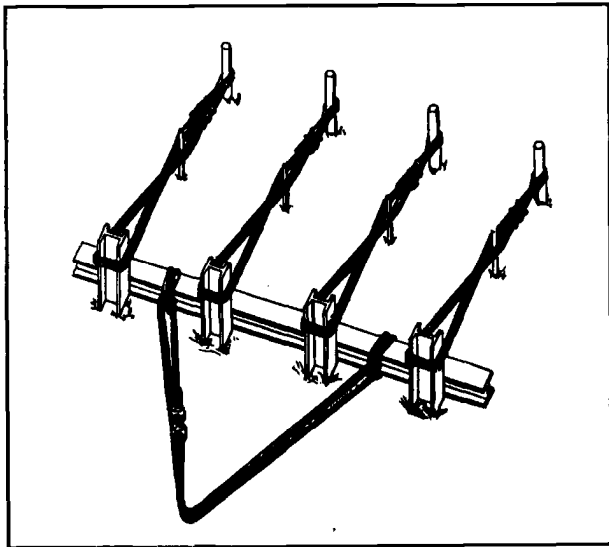
Figure 4-12. Combination steel picket holdfast
