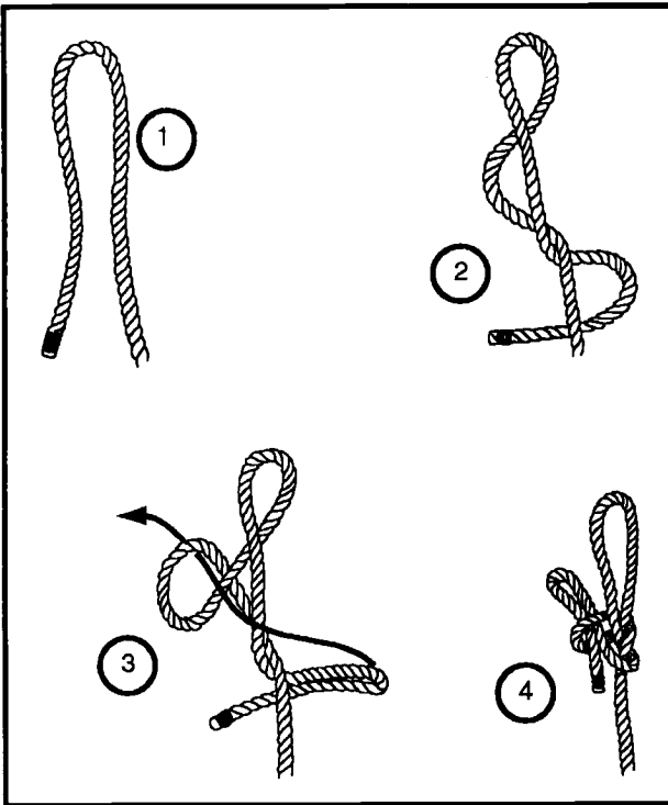
Figure 2-17. Speir knot
