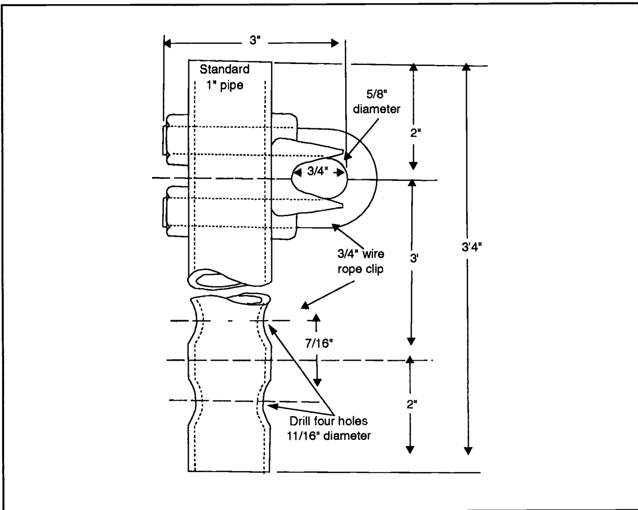
Figure 2-56. Iron-pipe stanchions
