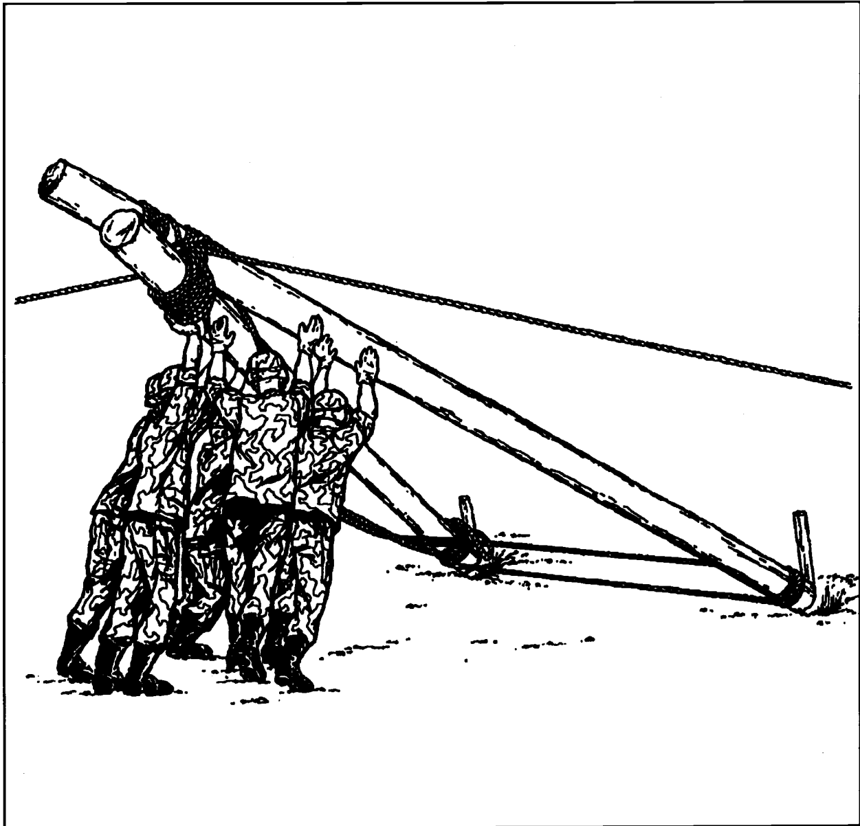
Figure 5-7. Erecting shears
