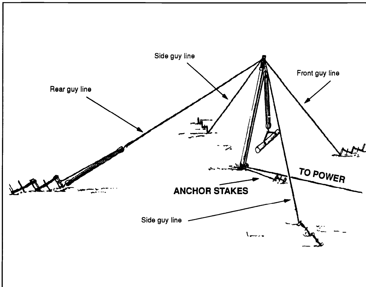
Figure 4-18. Typical guy-line installations
