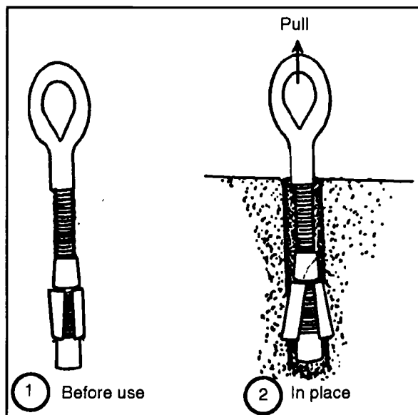
Figure 4-4. Rock anchor
