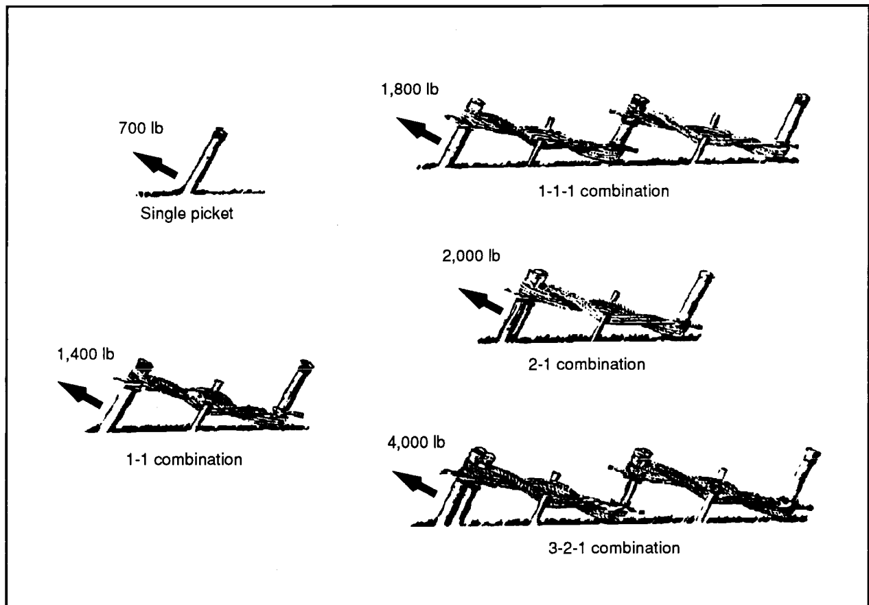
Figure 4-5. Picket holdfasts (loamy soil)
