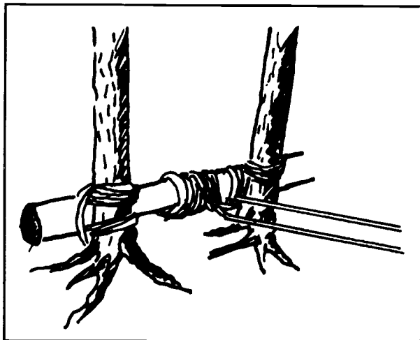
Figure 4-2. Natural anchorage (trees and transom)
