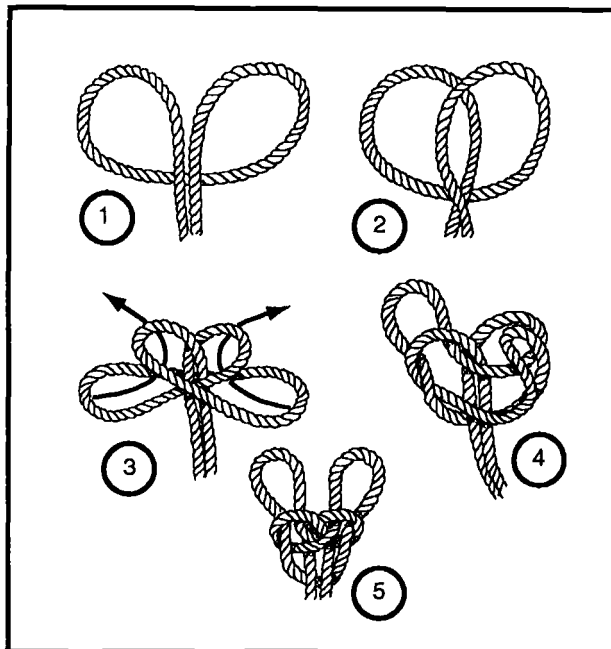
Figure 2-15. Spanish bowline
