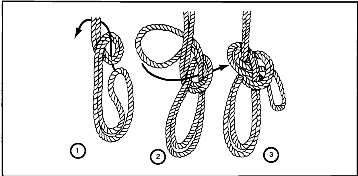
Figure 2-12. Double bowline
