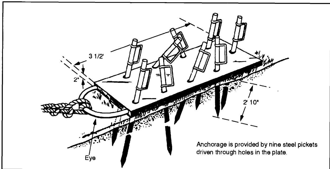
Figure 4-8. Standard steel-picket holdfast
