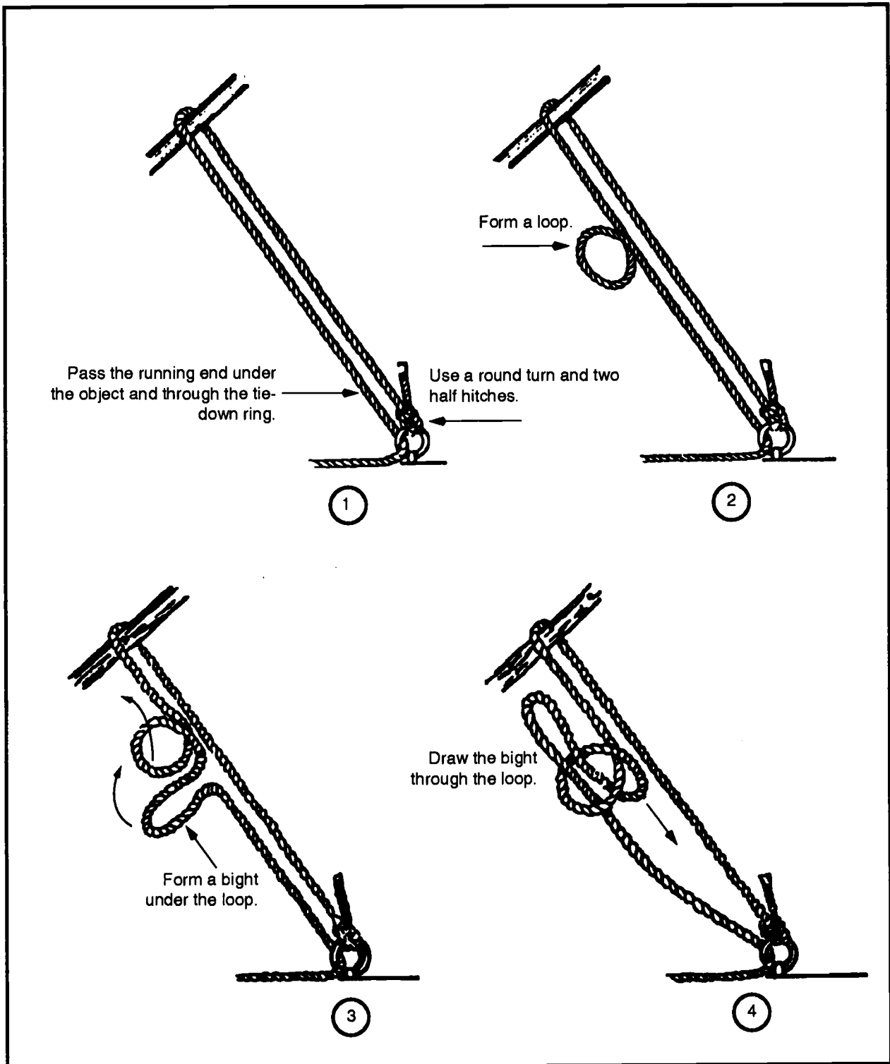
Figure 2-21. Baker bowline
