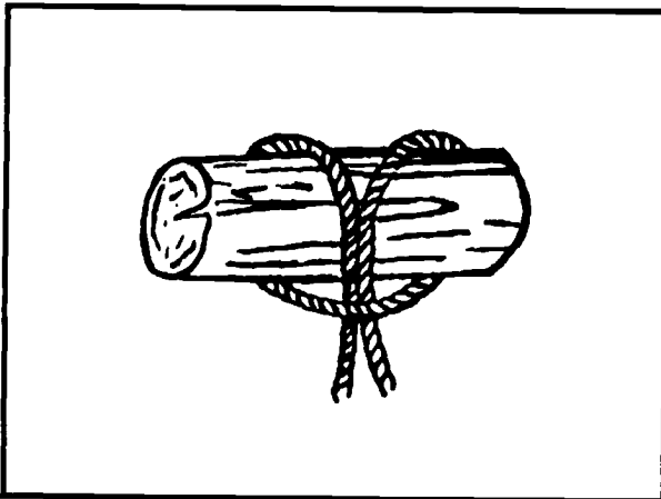
Figure 2-33. Girth hitch
