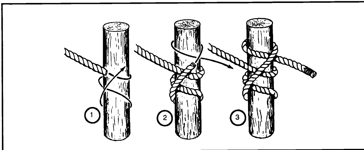
Figure 2-29. Mooring hitch
