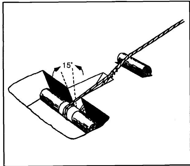
Figure 4-13. Log deadman
