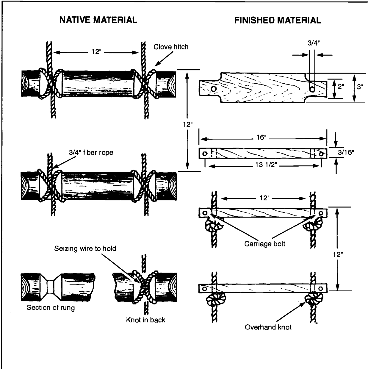
Figure 2-60. Wood rungs
