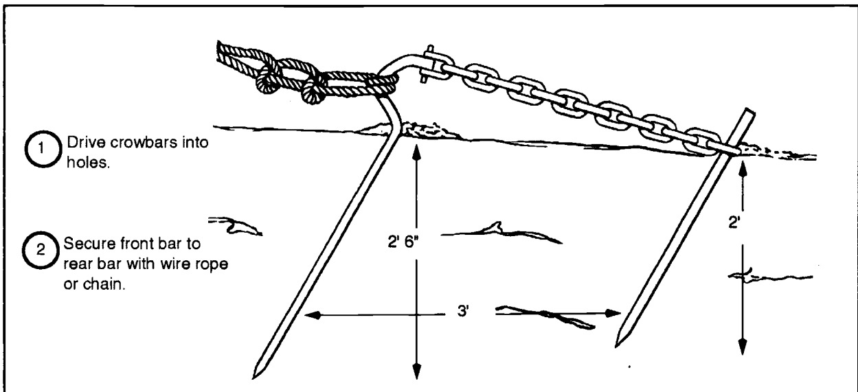
Figure 4-10. Rock holdfast
