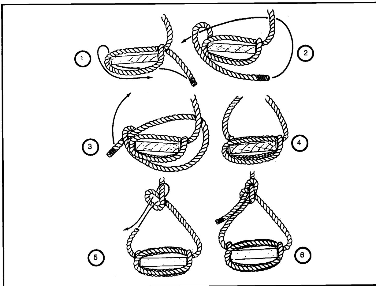
Figure 2-30. Scaffold hitch
