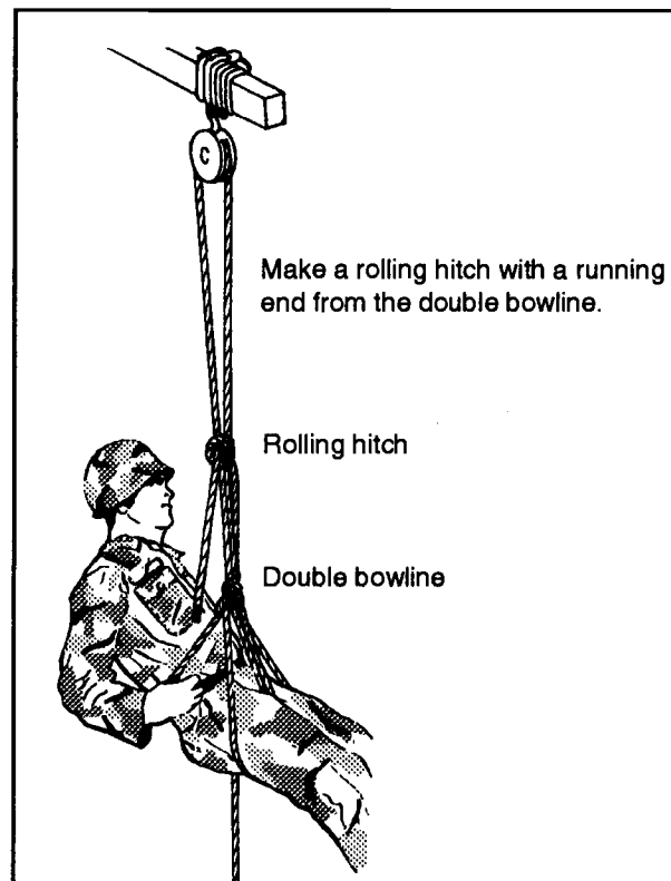
Figure 6-6. Boatswain's chair
