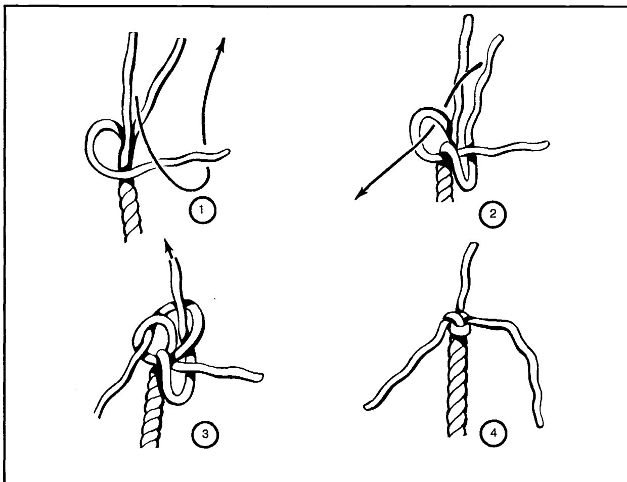
Figure 2-5. Wall knot
