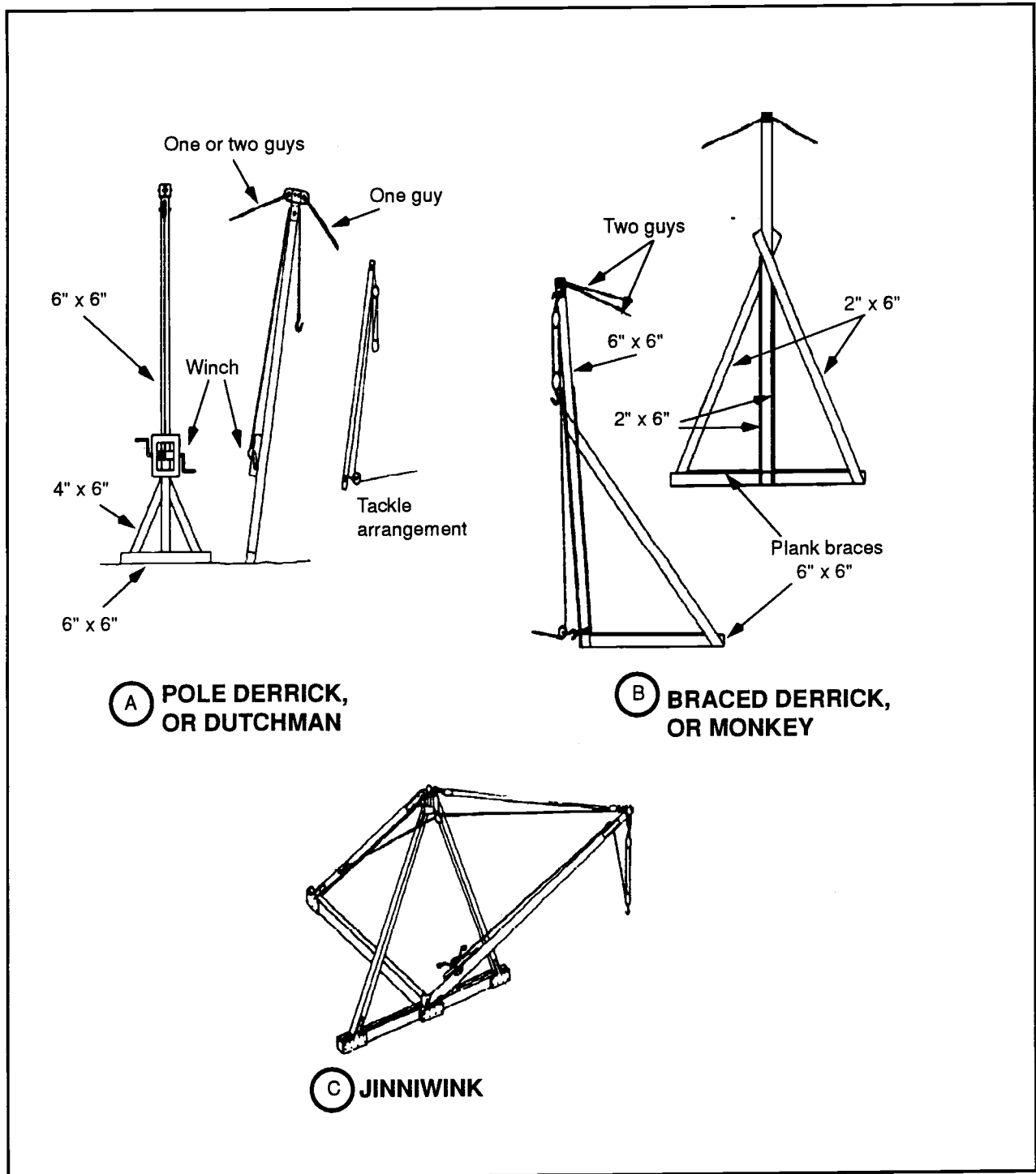
Figure 5-11. Light hoisting equipment
