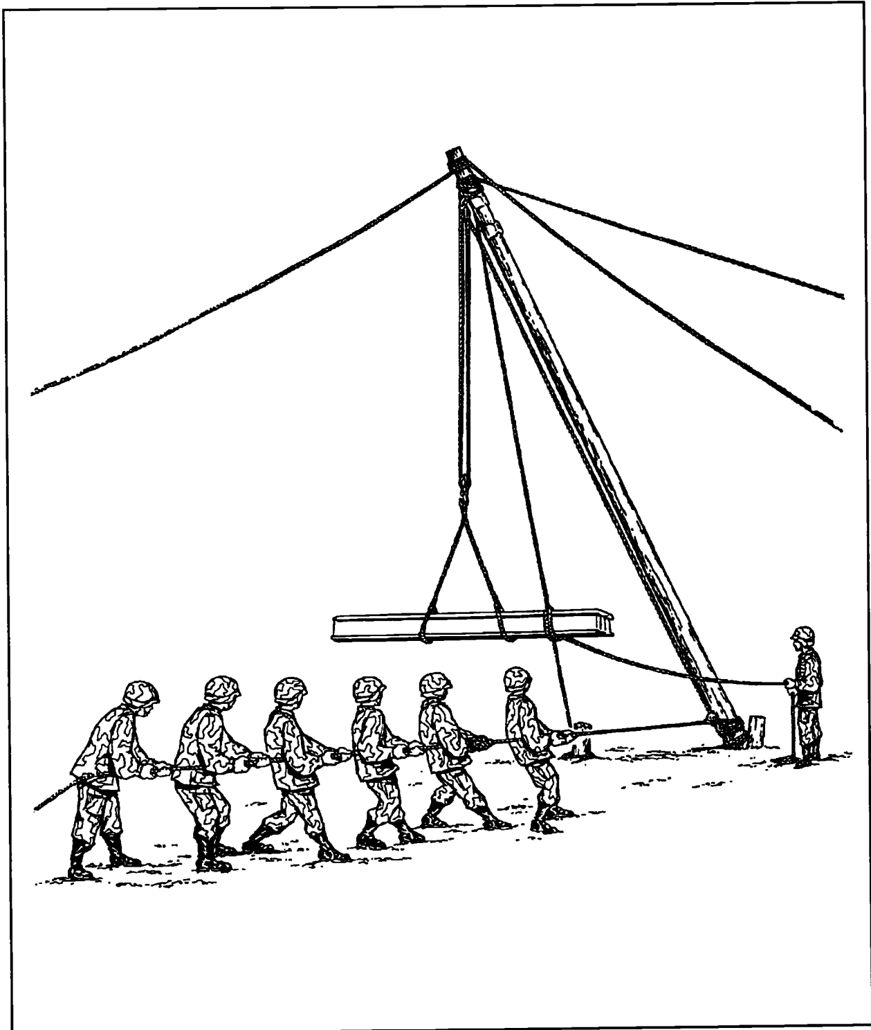
Figure 5-3. Hoisting with a gin pole
