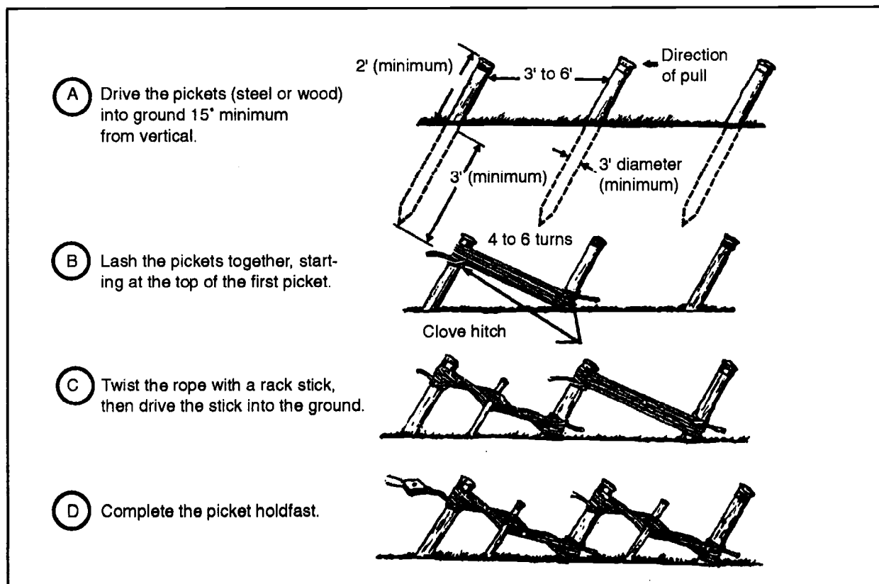
Figure 4-6. Preparing a picket holdfast
