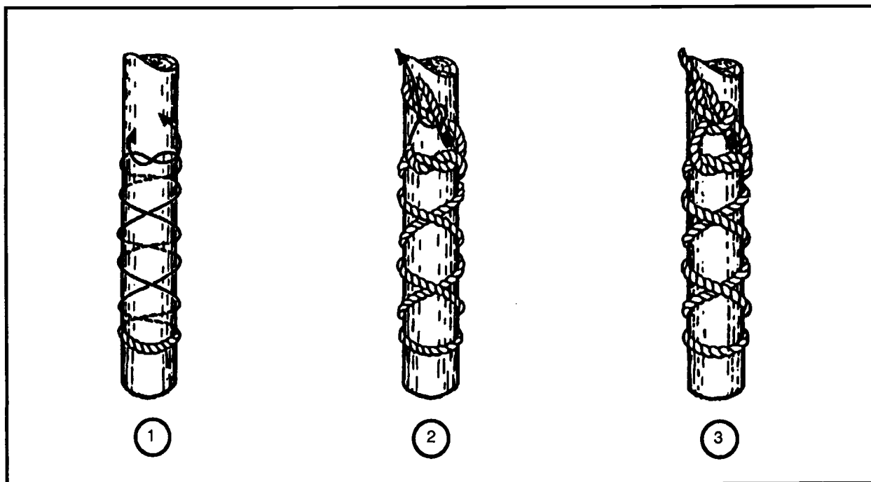
Figure 2-28. Telegraph hitch
