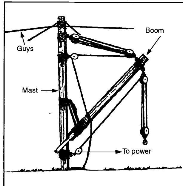
Figure 5-9. Rigging a boom on a gin pole
