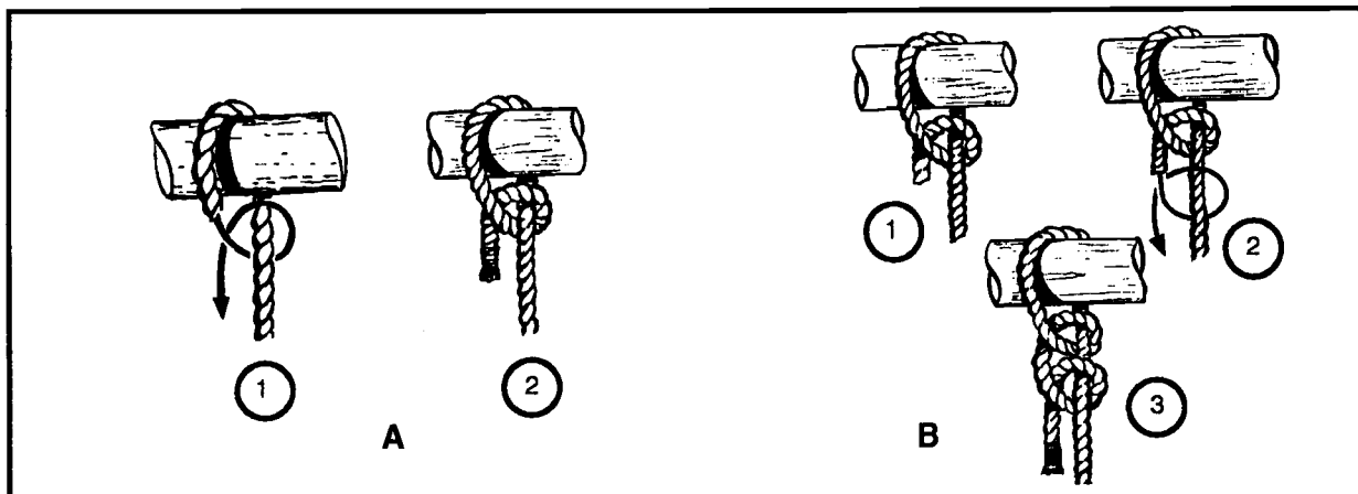
Figure 2-22. Half hitches
