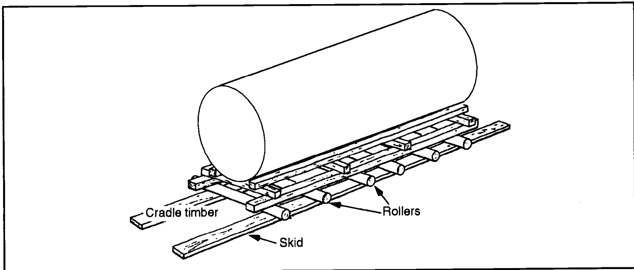
Figure 5-13. Using skids and rollers
