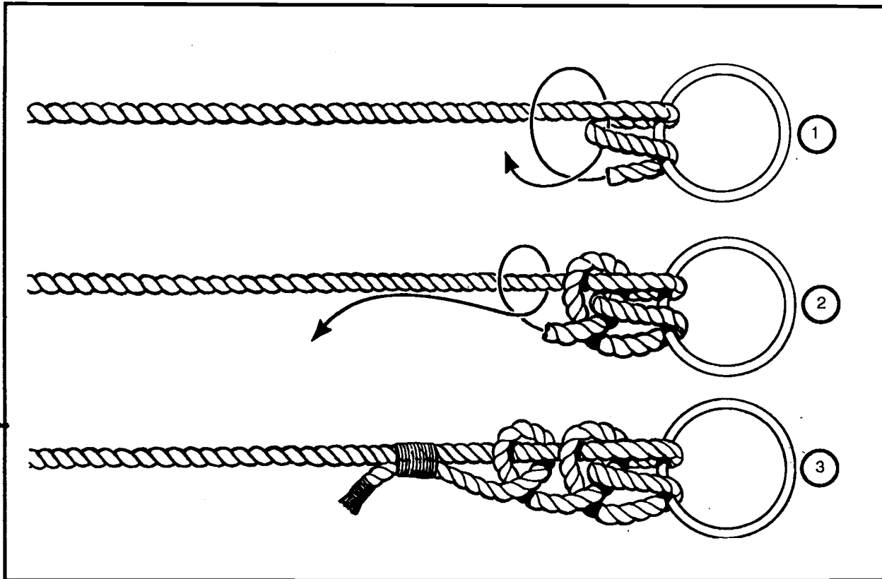
Figure 2-35. Fisherman's bend
