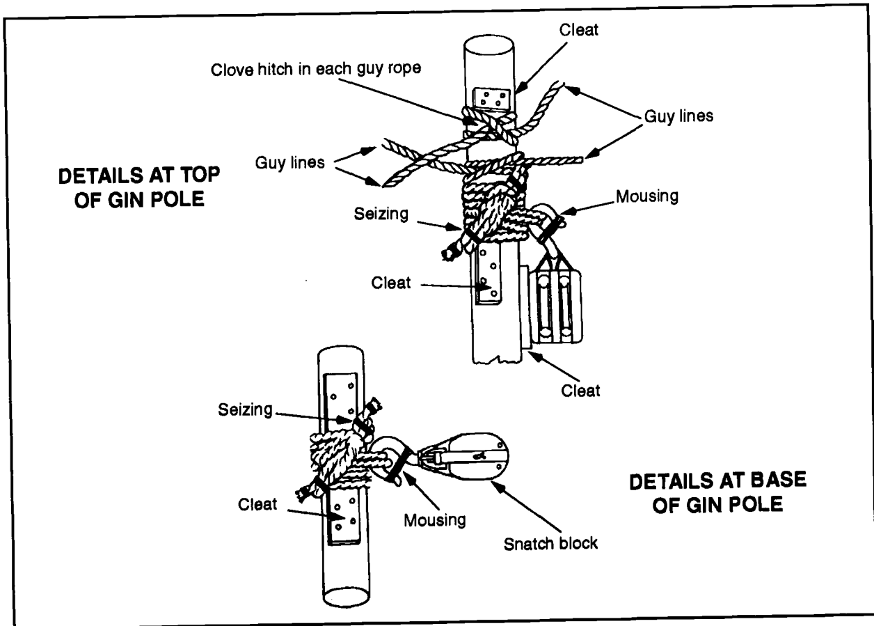
Figure 5-1. Lashing for a gin pole
