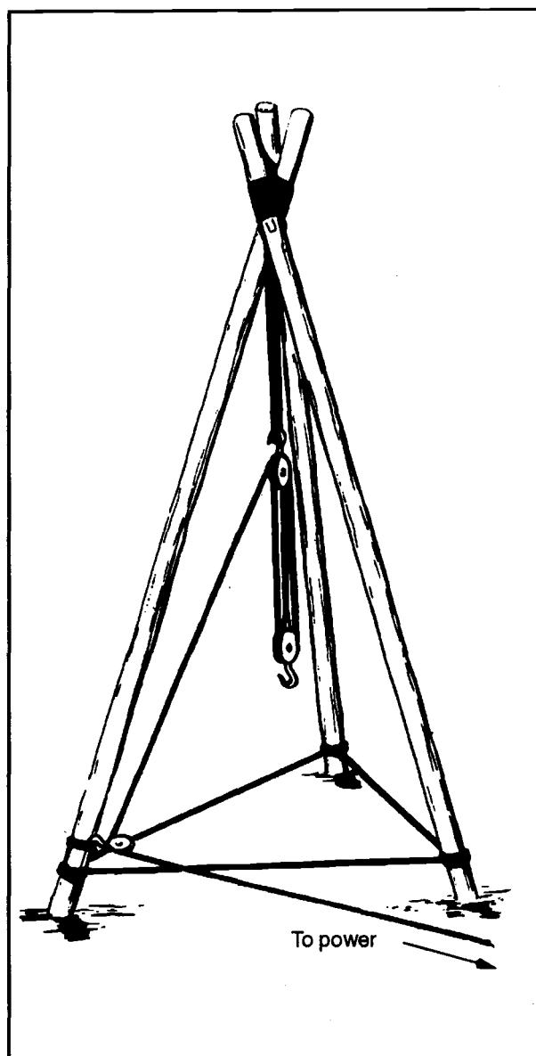
Figure 5-5. Assembled tripod
