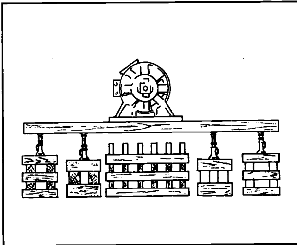
Figure 5-15. Jacking loads by stages
