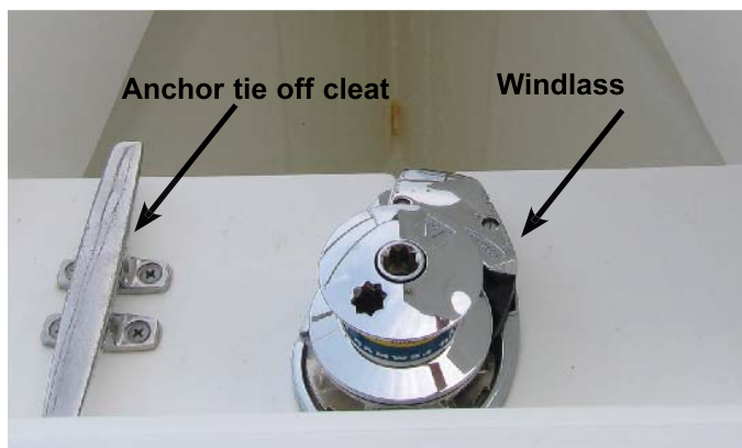
Figure 7.5 Anchor Well
