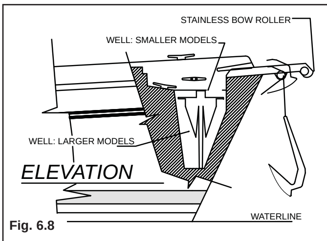
Fig 6.8 shows you a profile view of the anchoring. This illustration shows the smaller and the larger anchor well, in relation to the location.
