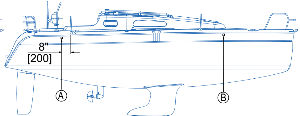
LIFTING POINTS FOR SAILDRIVE
