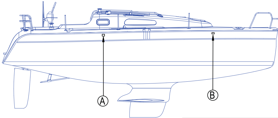
LIFTING POINTS FOR STERN DRIVE
