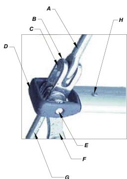
UPPER SPREADER TIP
