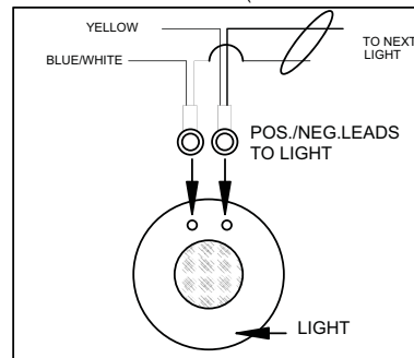
EXAMPLE LIGHT WIRING (PARALLEL CIRCUIT)
