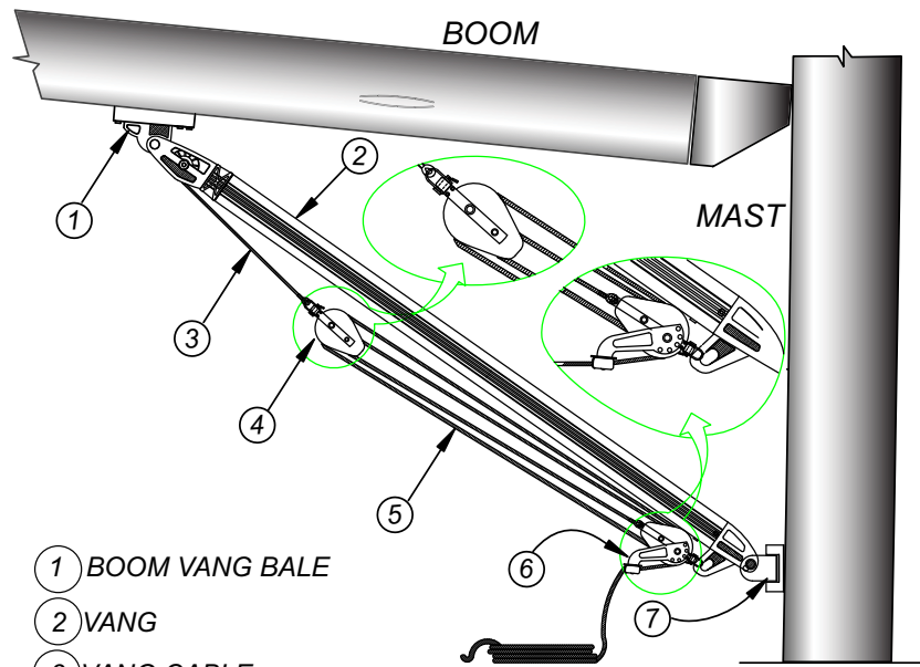
TYPICAL RIGID VANG DETAILS (FURLING OPTION)
