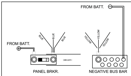
EXAMPLE SWITCH PANEL WIRING (PARALLEL CIRCUITS)
