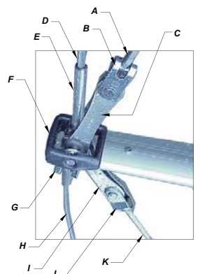
LOWER SPREADER TIP
