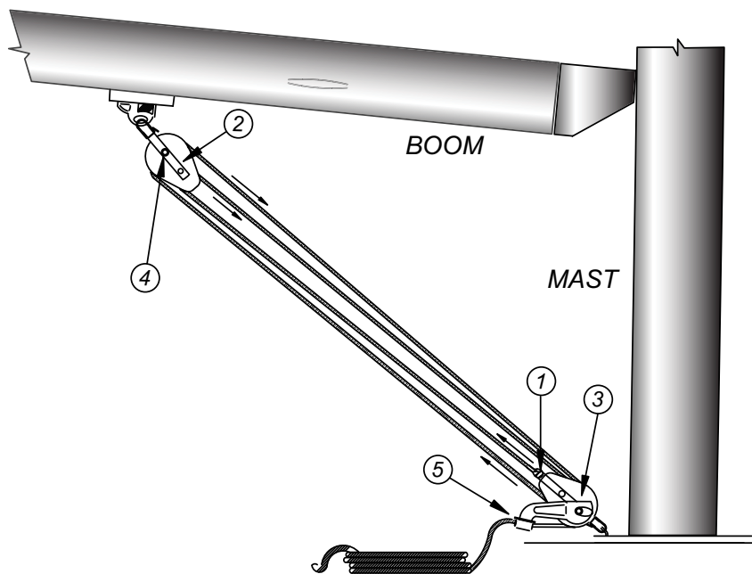
TYPICAL ROPE VANG DETAILS (STANDARD)
